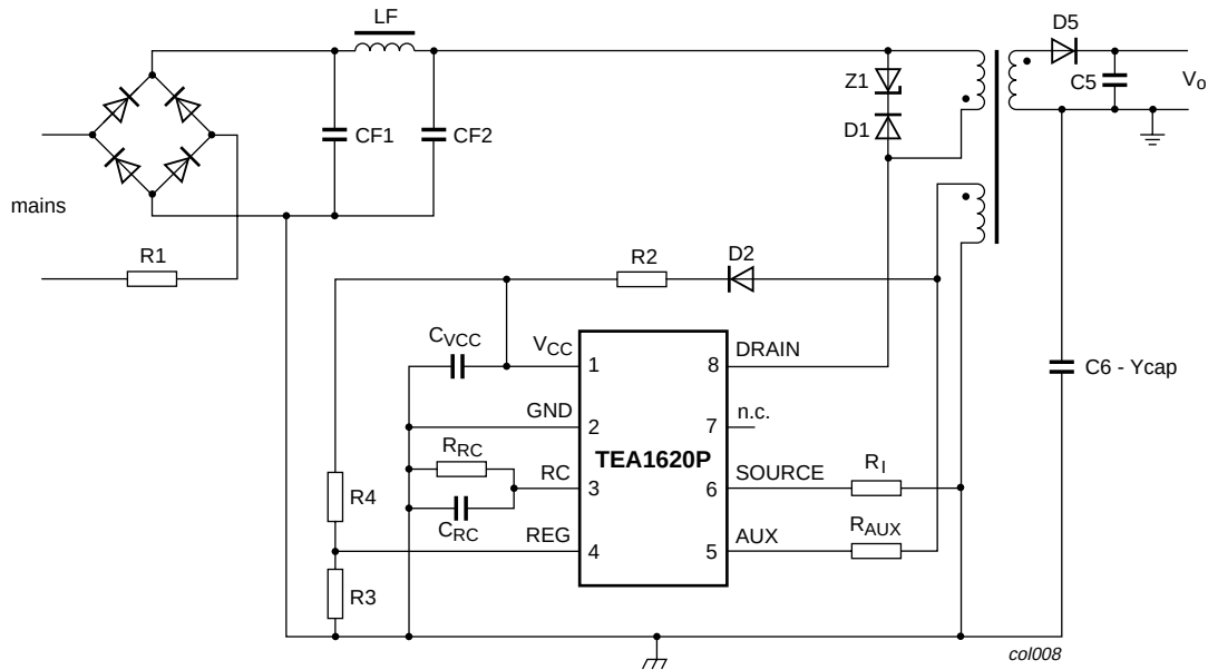
Fig 5. Application with primary sensing.
